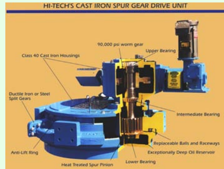
Drive unit
